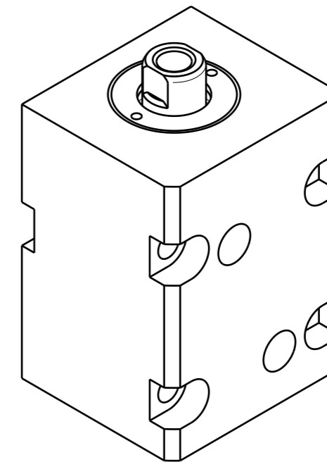
Isometric view (1:1)
