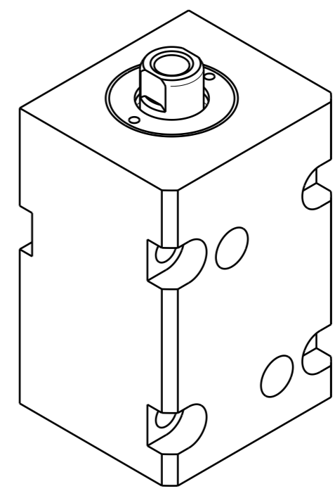
Isometric view (1:1)
