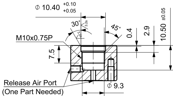
<MOUNTING DIMENSION>
