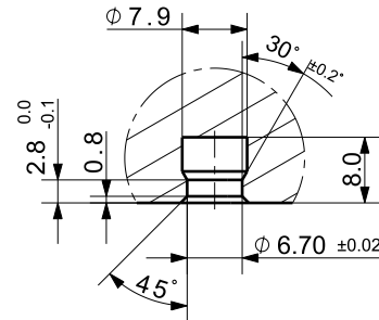
<Workpiece Hole Reference Dimensions>
