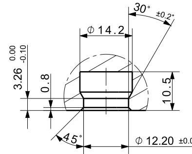
<Workpiece Hole Reference Dimensions>
