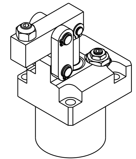
Isometric view (1:2)
