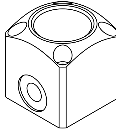
Isometric view (1:1)
