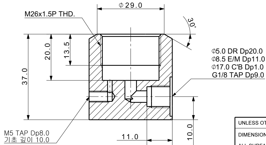
Section view A-A (1:1)
