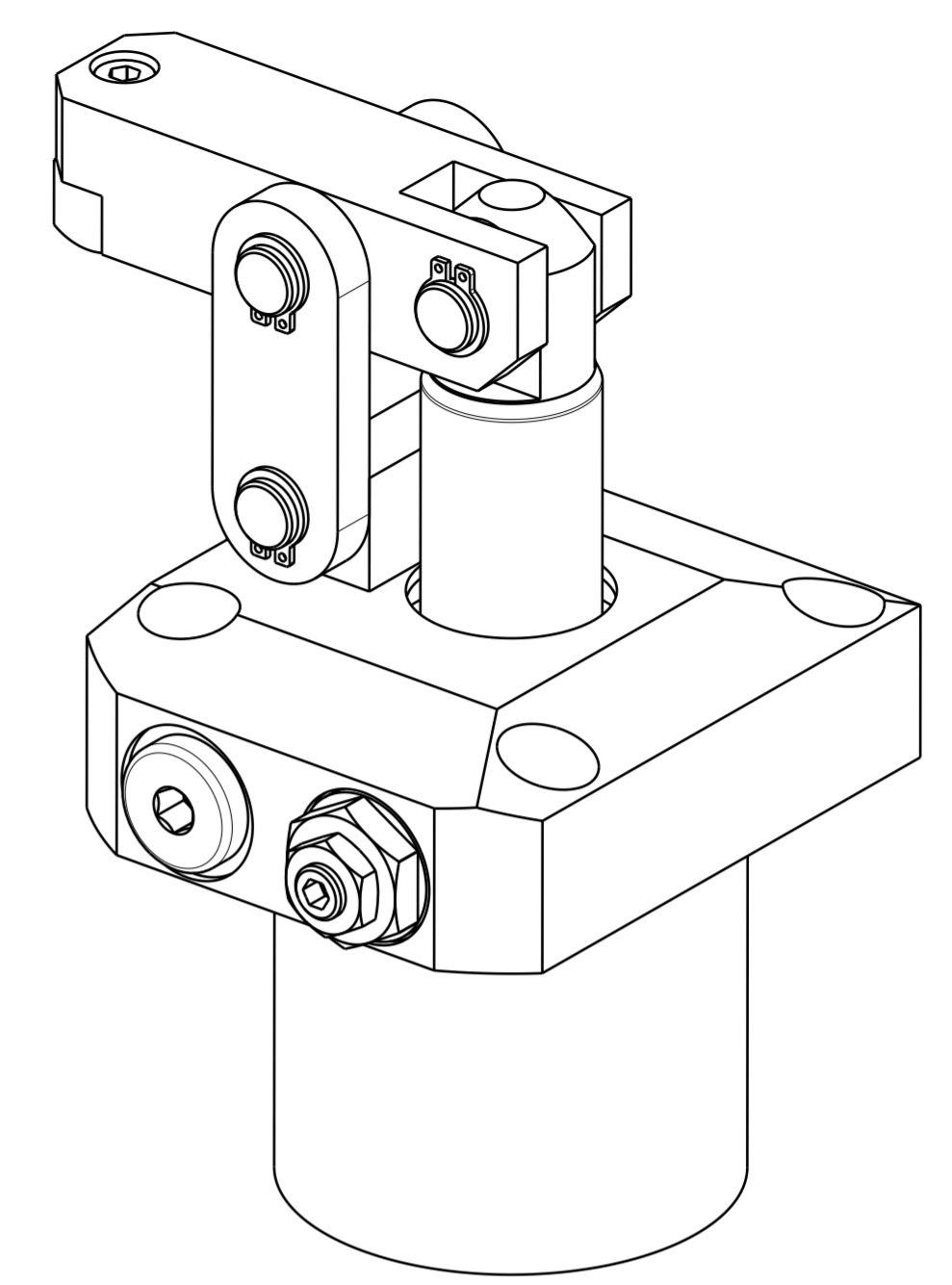
Isometric view (1:1)
