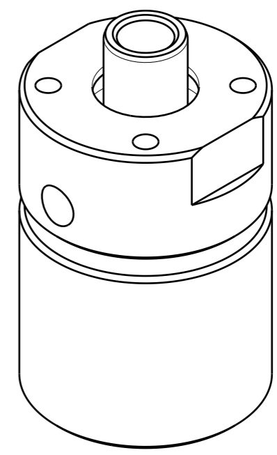
Isometric view (1:1)
