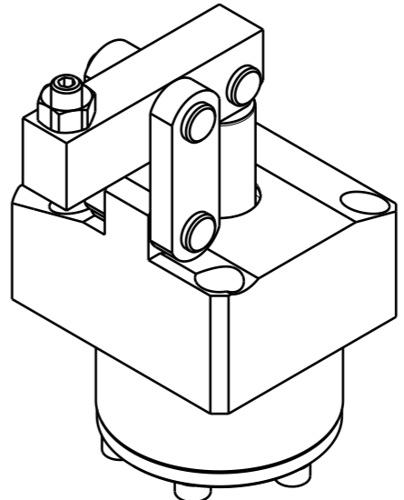
Isometric view (3:4)
