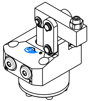
Isometric view (1:2)
