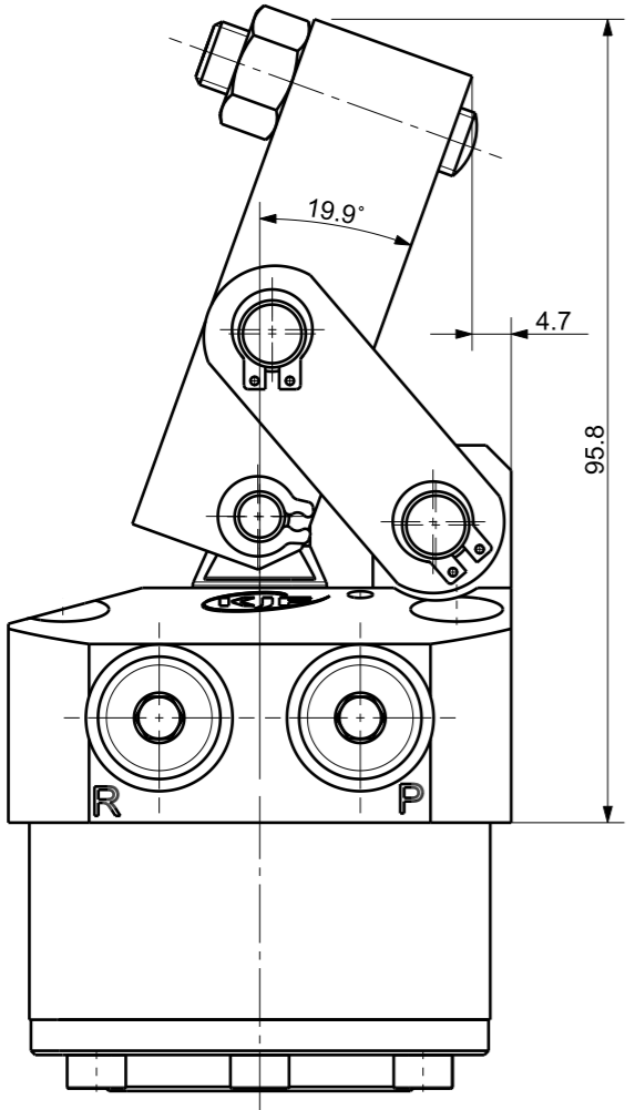
VIEW "B"
