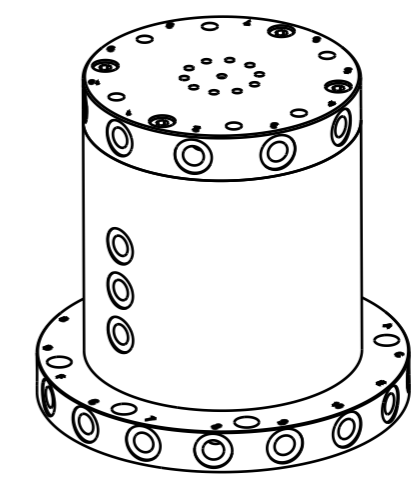
Isometric view (1:4)
