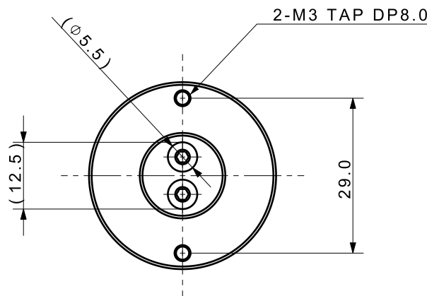
View "A" (1:1)
