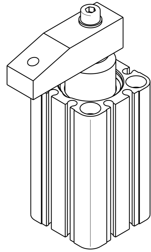
Isometric view (1:1)
