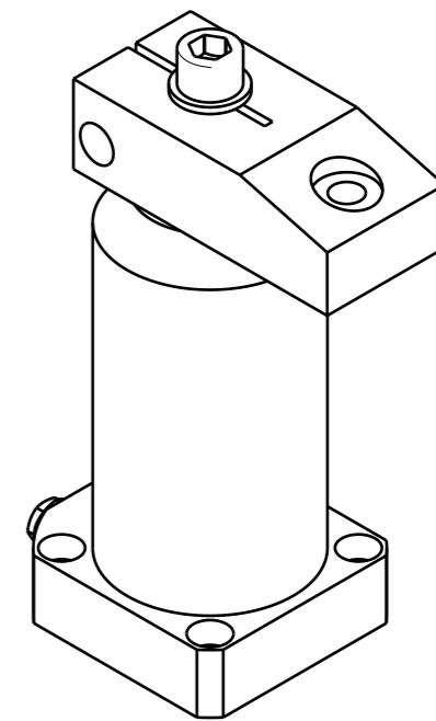
Isometric view (1:3)
