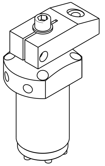
Isometric view (1:3)
