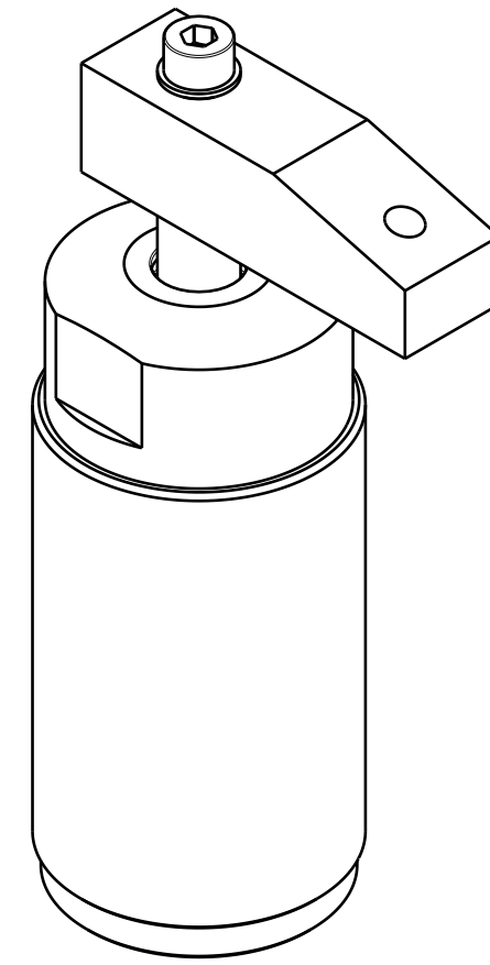
Isometric view 1:1
