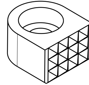
Isometric view (2:1)
